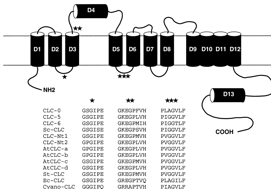
Fig. 4. Topology model for the animal chloride channels (from [116]) and sequence alignment for three conserved domains (stars) in animal, yeast, plant and bacterial CLCs. CLC-0, Torpedo marmorata ; CLC5 and CLC6, rat; ScCLC, Saccharomyces cerevisiae ; CLC-Nt1 and CLC-Nt2, Nicotiana tabacum ; AtCLC-a to -d, Arabidopsis thaliana ; St-CLC, Solanum tuberosum ; Ec-CLC, Escherichia coli ; Cyano-CLC, Synechocystis sp.
